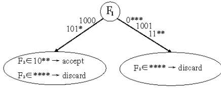
Fig. 4. “Virtual” one-dimensional packet classifier
