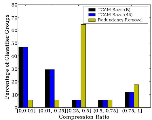
Fig. 7. Distribution of real-life packet classifiers by compression ratio
