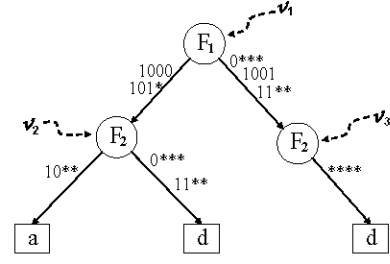
Fig. 3. A packet classifier decision diagram
