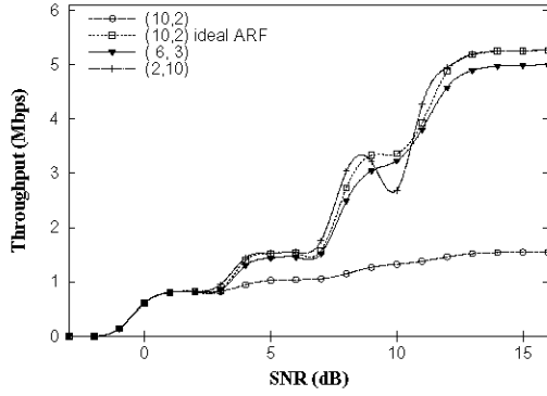
Fig. 6. ARF-DCF throughput for various \theta_u, \theta_d combinations under N = 5
