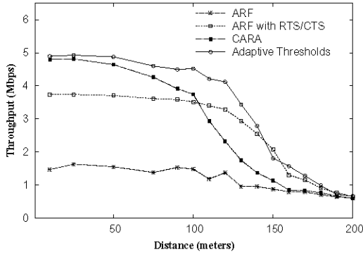
(b) N=5
