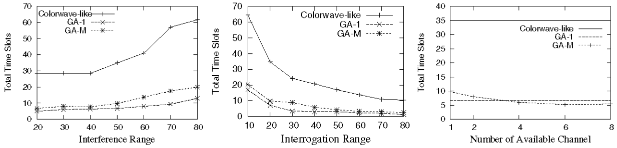
Fig. 4. Performance of the GA-1, GA-M, and Colorwave-like algorithms for the MCS problem. (a) Varying interference range with single channel, (b) Varying interrogation range with single channel, and (c) Varying number of available channels.
