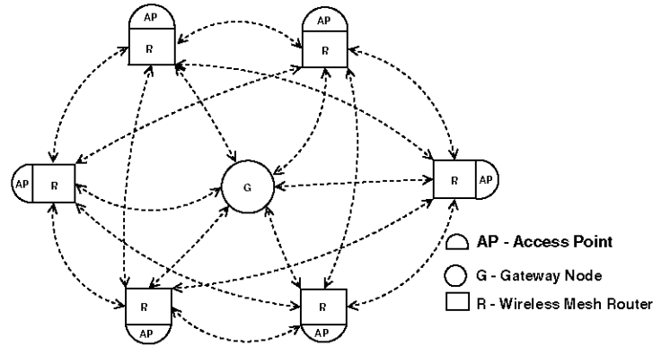
Fig. 1. Hierarchical structure of wireless mesh access networks.
