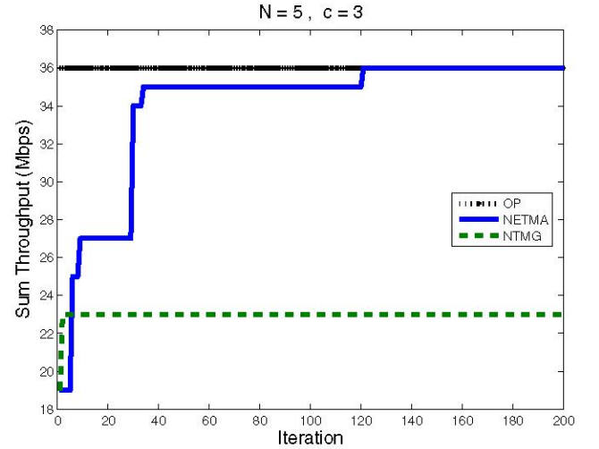
Fig. 4. Performance evaluation of the wireless mesh access network with N = 5 and c = 3 .
