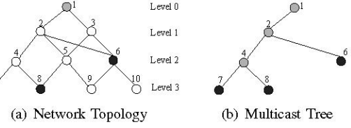
Fig. 4. A Multicast Structure Example
