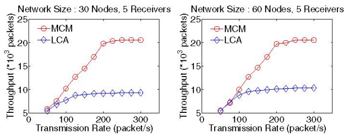
Fig. 9. Impact of Number of Transmission Rate
