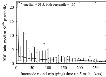
Figure 9. Tapestry Performance. Relative Delay Penalty (RDP) for packets routing the Tapestry network on the PlanetLab network testbed. Tapestry provides relatively low overhead compared to IP in the wide area.
