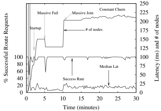
Figure 21. Pair-wise Routing with Self-Repair. Success rate of Tapestry routing between random pairs of nodes with self-repair enabled during massive failure, massive join, and constant churn conditions.
