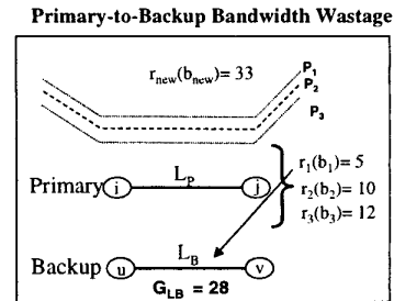
Figure 2. Primary-to-Backup Link Wastage
