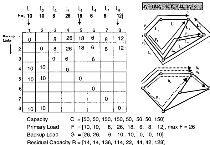
Figure 3. Example of a BLD matrix
