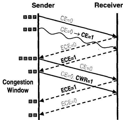
Figure 1. ECN avoids dropped packets by allowing routers to signal congestion by setting the Congestion Experienced (CE) bit in the IP header. In TCP, the receiver returns congestion signals by setting the ECN-Echo (ECE) flag. The sender sets the Congestion Window Reduced (CWR) flag to inform the receiver that it has reacted to congestion.
