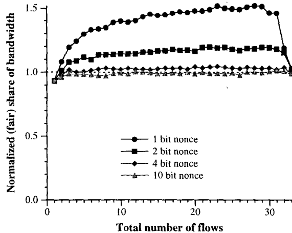
Figure 7. Misbehavior is detected by 1, 2, 4 and 10-bit nonces. When misbehavior is detected, the congestion window is reduced by one-half. A 10-bit nonce closely approximates a true ECN signal, while 4, 2, and 1-bit nonces allow the misbehavior to gain progressively more bandwidth.
