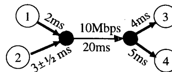
Figure 3. The simulated network topology is shown. Arrows represent the direction of traffic flow. Links other than the bottleneck are 100Mbit/s. The link to Node 2 has a one way latency randomly chosen uniformly between 2.5 and 3.5ms. Several traffic sources or sinks were placed on each node to vary congestion at the bottleneck.
