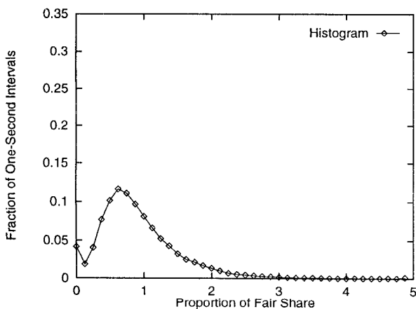
Figure 4: Fairness Histogram for 30 Flows
