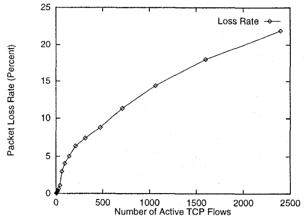
Figure 7: Number of Flows vs. Loss Rate
