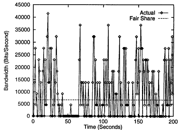
Figure 5: Bandwidth of One of the 1500 Flows
