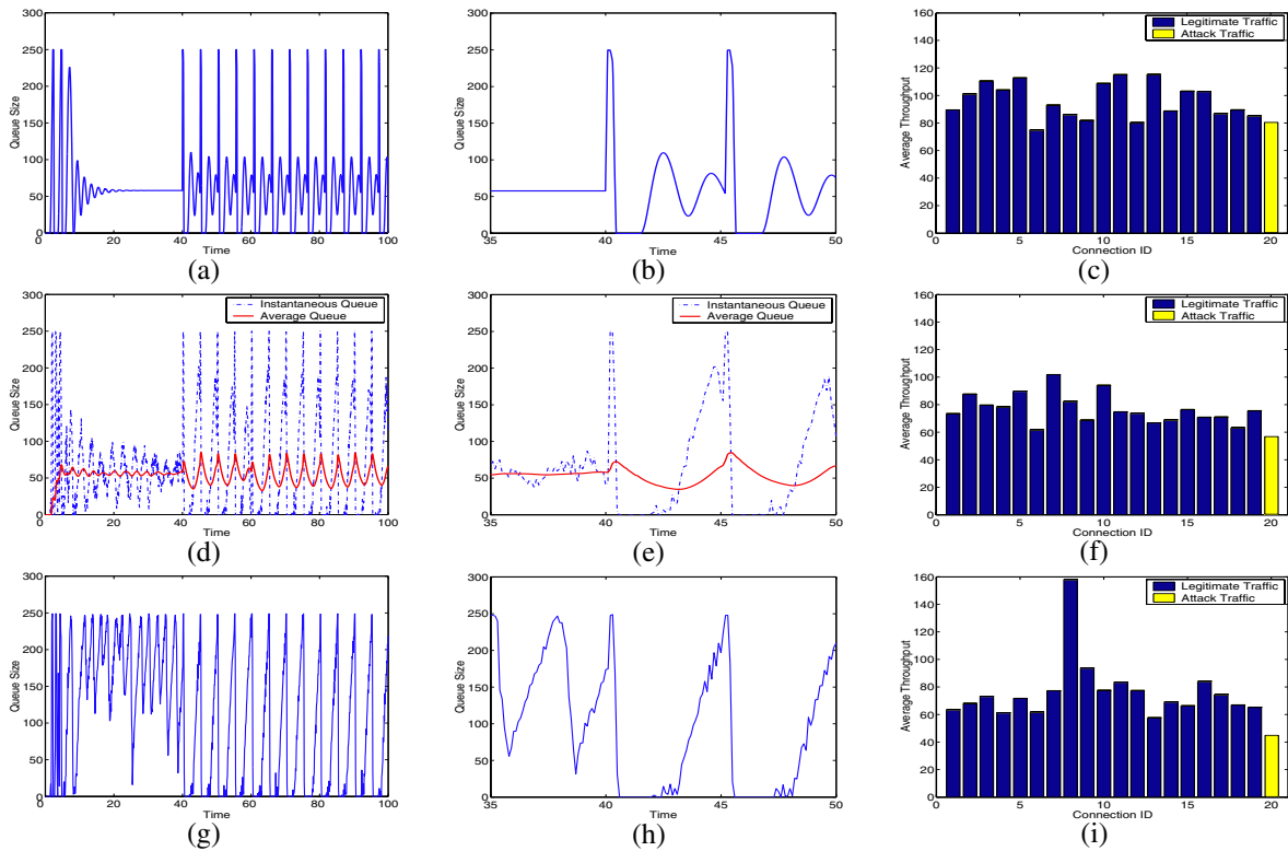
Figure 4. Vulnerability to RoQ attacks: Queue size over time (left and center) and throughput achieved per flow in the presence of attack (right). Top row shows results predicted by analytical model of TCP+RED; middle row shows ns simulation results with RED queue; bottom row shows ns simulation results with DropTail queue.
