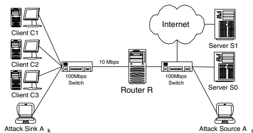
Figure 6. Setup for Internet Experiments.
