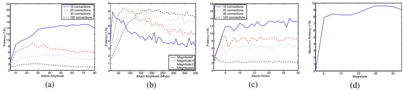
Figure 5. Tuning attack parameters to maximize potency (for link bandwidth) using \Omega = 1 : Effect of changing \delta for a fixed magnitude ( M = 5 ) under different number of flows (a). Effect of changing \delta for a fixed number of 20 flows under different attack magnitudes (b). Effect of changing T for a fixed magnitude ( M = 5 ) with corresponding optimal \delta under different number of flows (c). Effect of changing M with corresponding optimal \delta and T (d).
