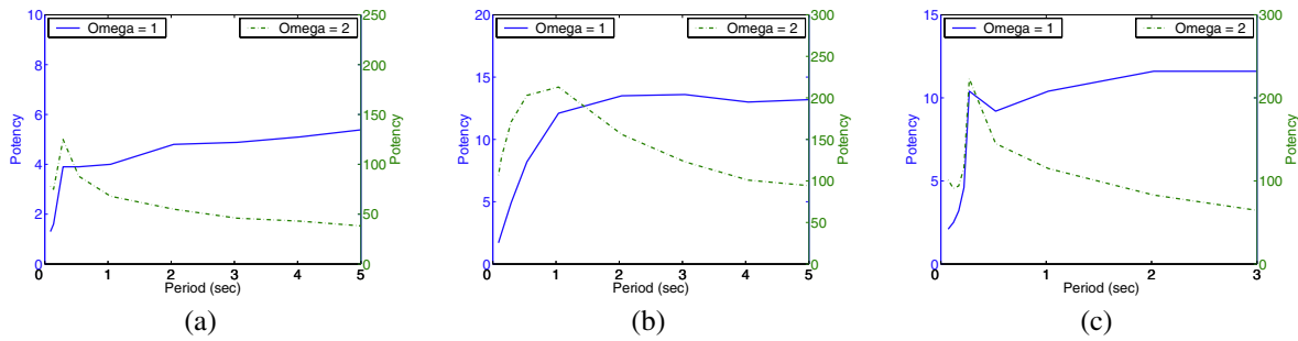
Figure 7. Potency of Internet RoQ attack as the attack period T (in seconds) is changed while keeping the attack duration \tau constant. Two potency curves are shown one for \Omega = 1 (labels on left y-axis) and one for \Omega = 2 (labels on right y-axis). Results shown are for (a) RoQ attack on flows with short RTTs with \tau=40\text{msec} , (b) flows with long RTTs with \tau=40\text{msec} , (c) a mix of long and short RTT flows with \tau = 20\text{msec} .
