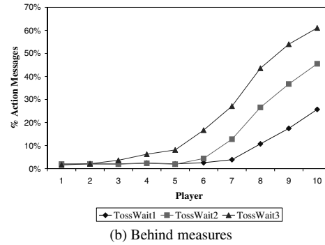
Figure 8. TossWait performance (with exact delay information used in Sync-out and estimated delay information used in Sync-in)
