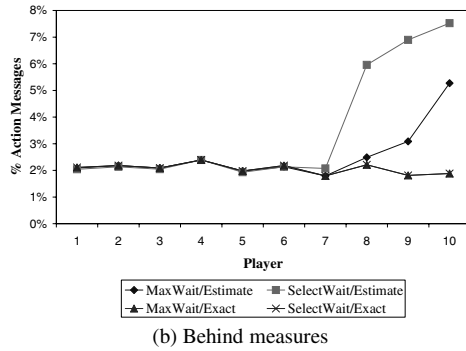
Figure 7. SelectWait vs. MaxWait (with exact delay information used in Sync-out)
