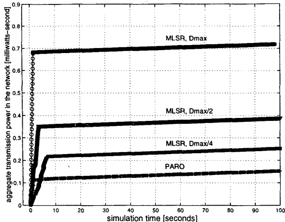
Figure 7. Aggregated Transmission Power Consumed by Data and Signaling for PARO and MLSR
