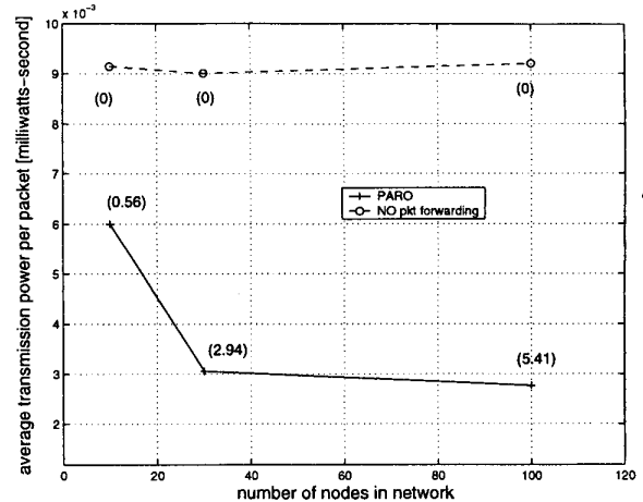
Figure 5. Transmission Power versus Average Number of Redirectors
