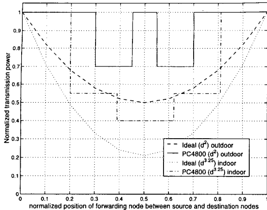
Figure 8. Experimental Results for Transmission Power versus the Position of a Redirector between a Source-Destination Pair for Indoor and Outdoor Environments
