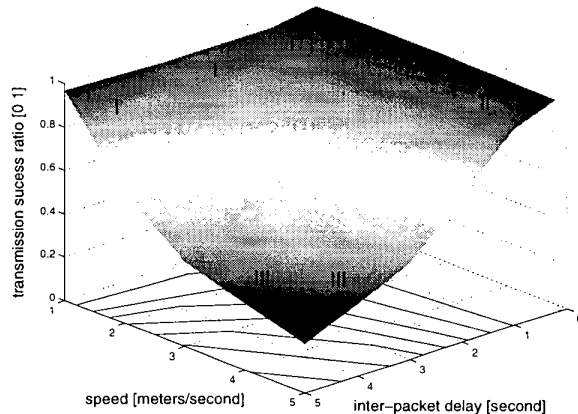
Figure 6. Transmission Success Performance
